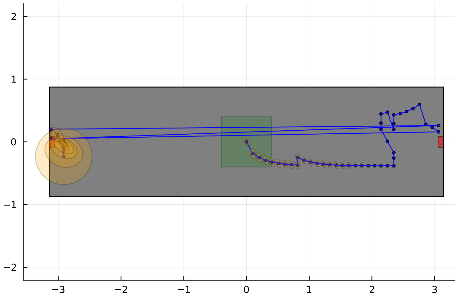
articulated_vehicle (theta,phi)
