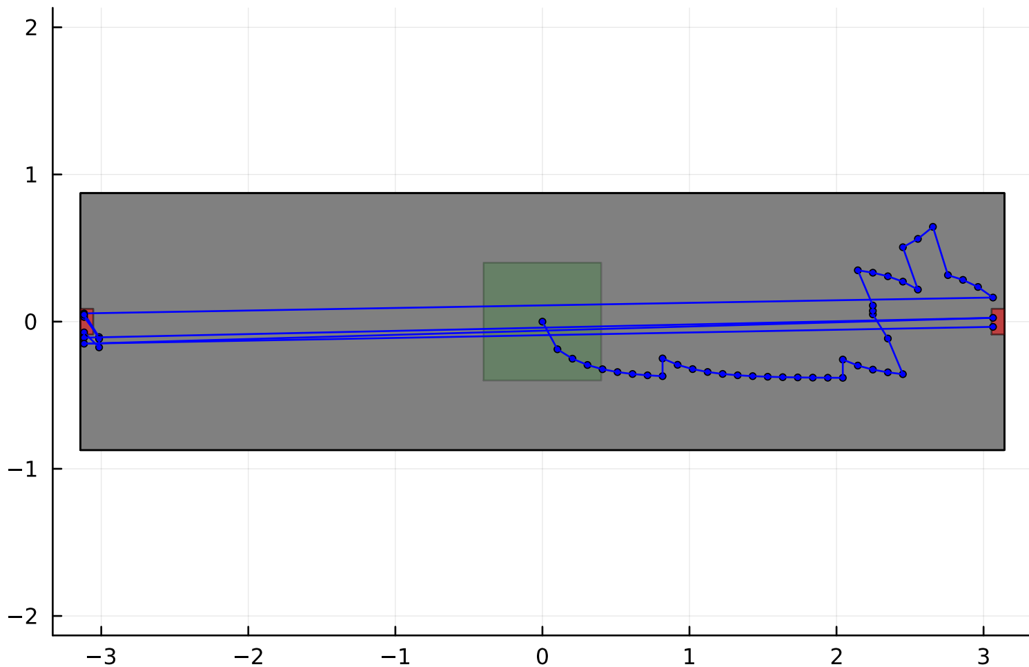
state_space_34 + ellipsoids
