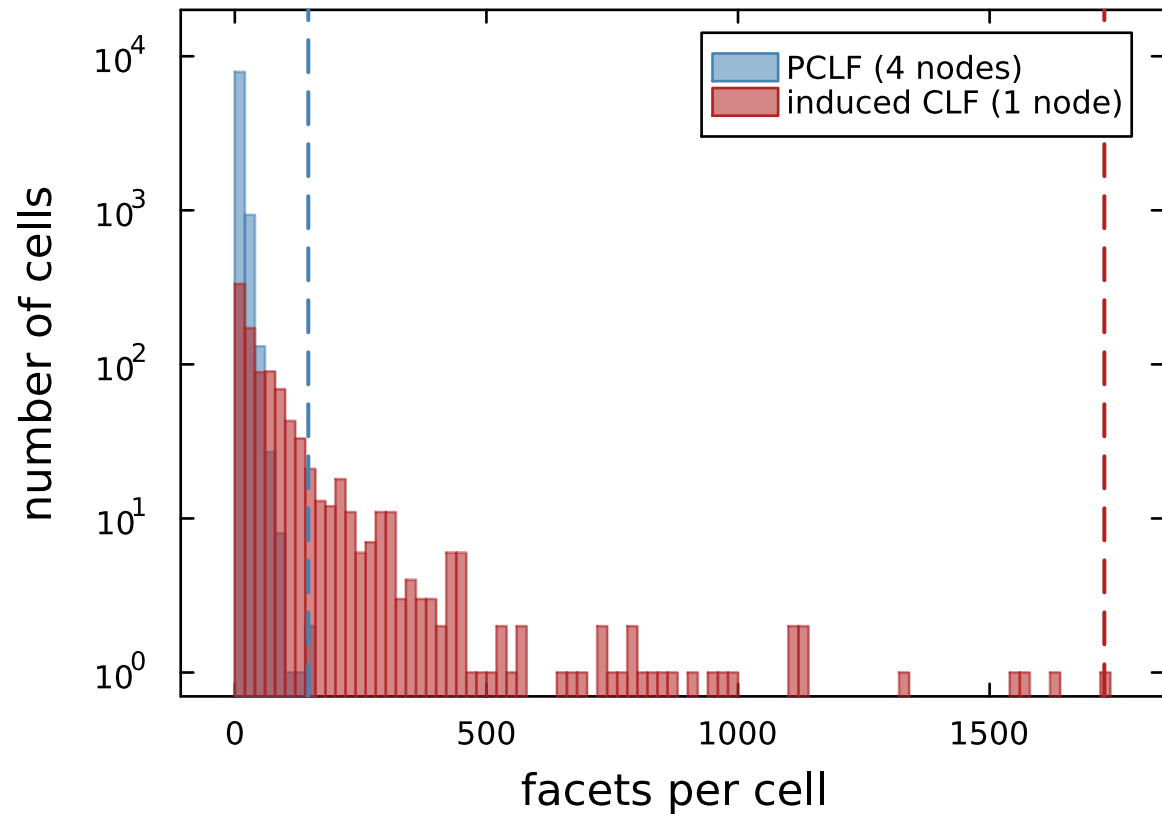
Facets per semilinear cell
