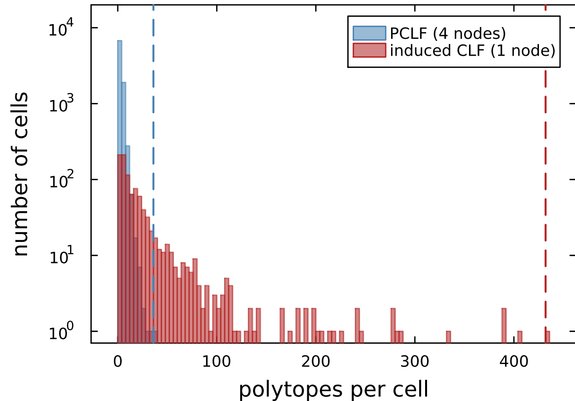
Pieces per semilinear cell
