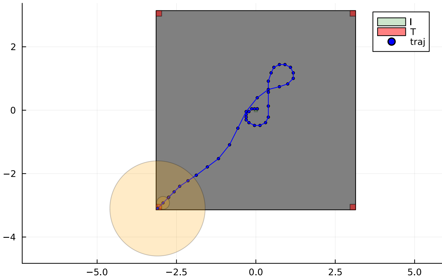
double_pendulum - (theta1, theta2)
