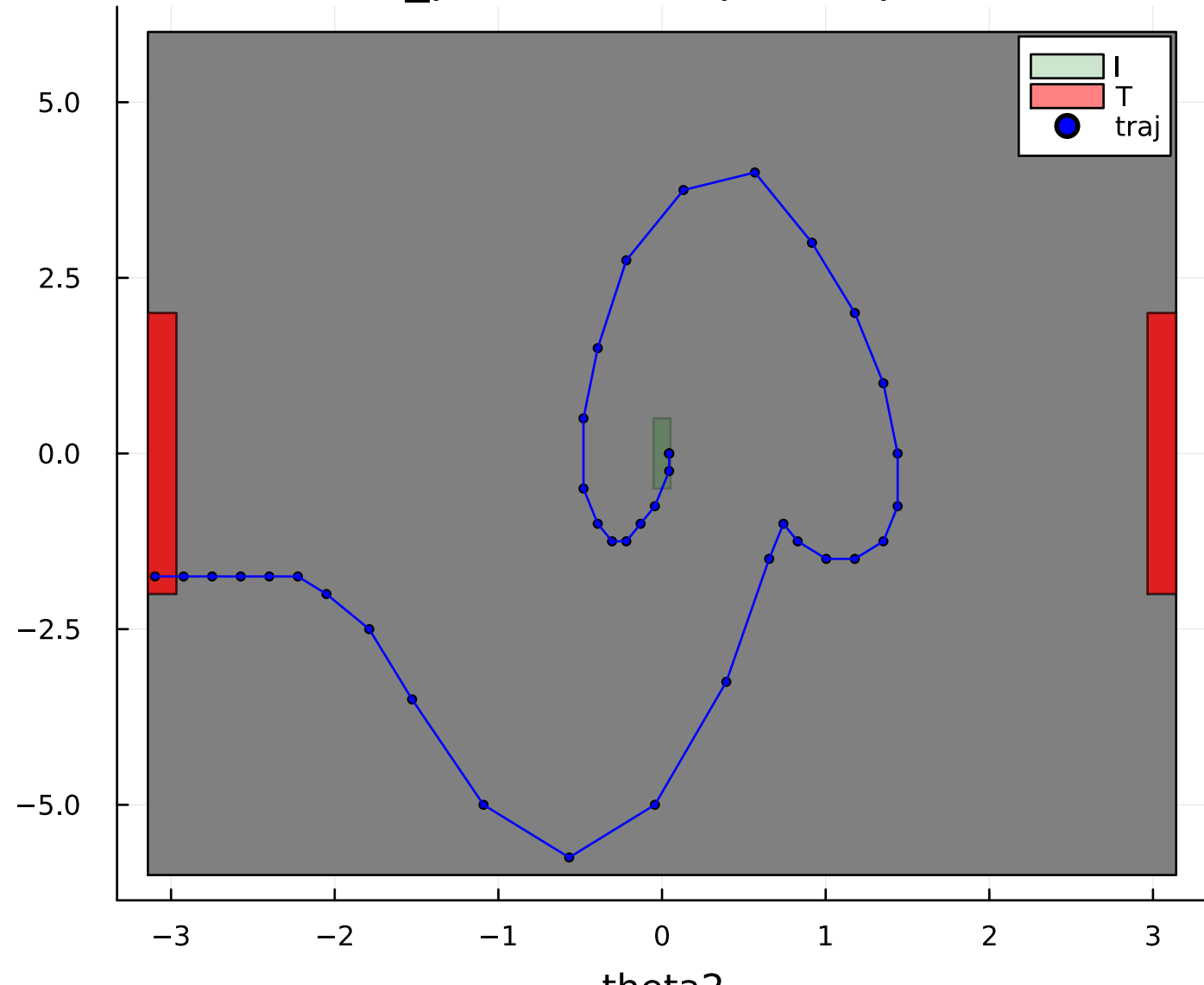
double_pendulum - phase portraits
