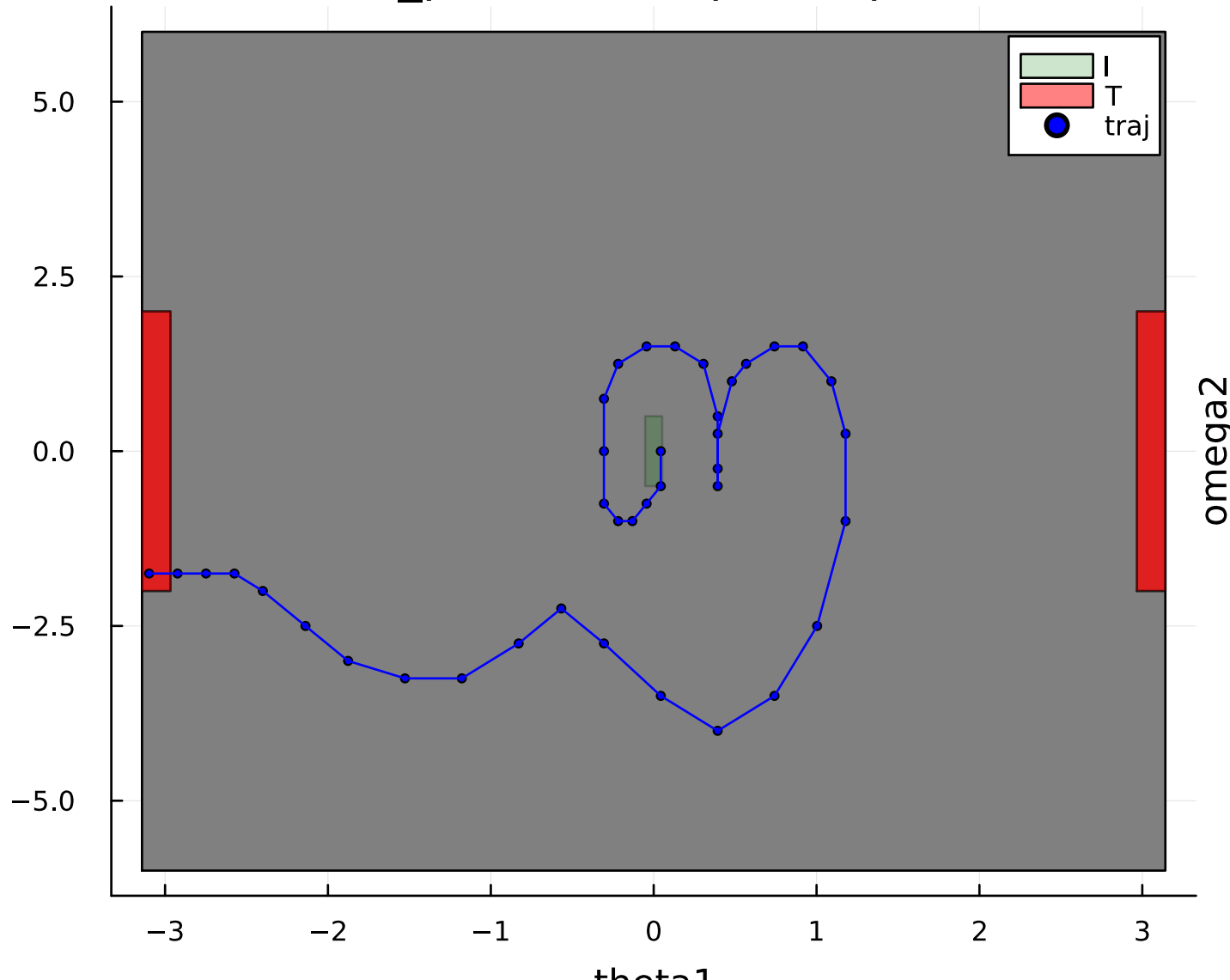
double_pendulum - phase portraits
