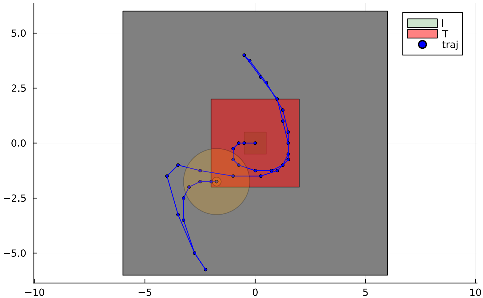
double_pendulum - ( \omega_1 , \omega_2 )
