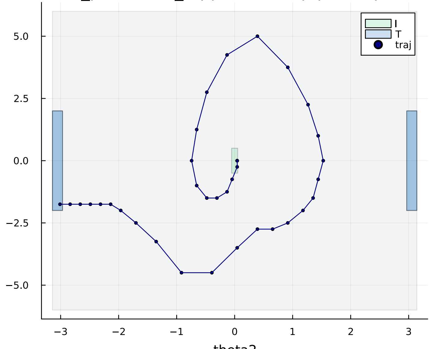
double_pendulum_mppi - warmup phase portrait
