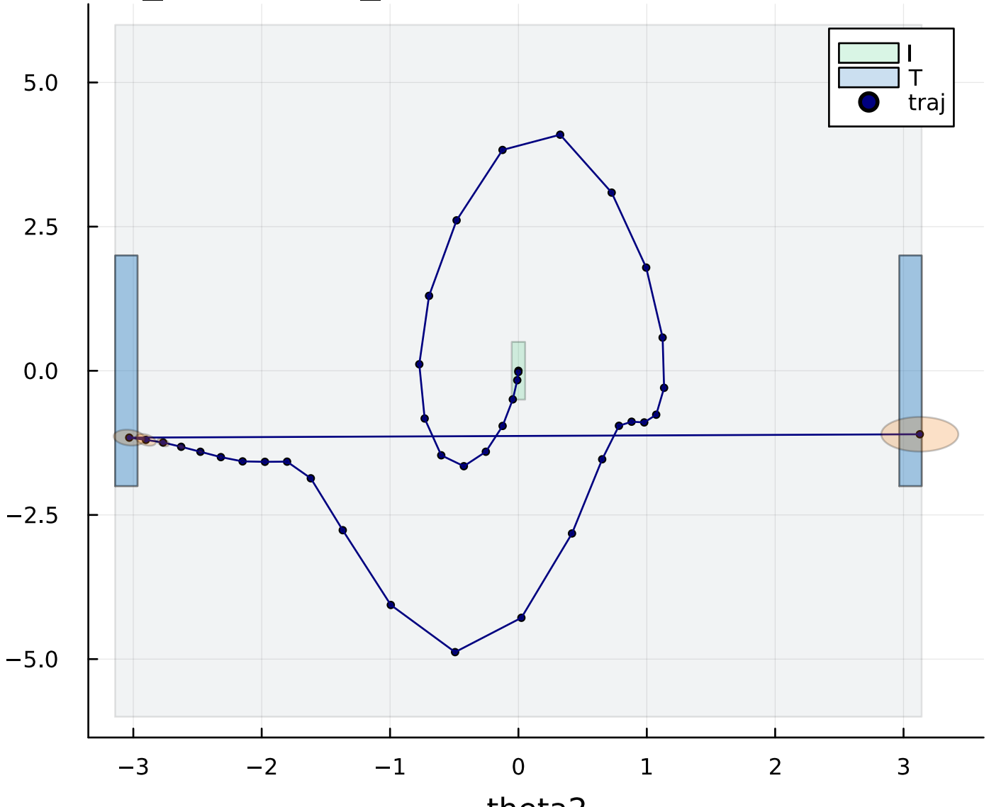
double_pendulum_mppi - certification phase portraits
