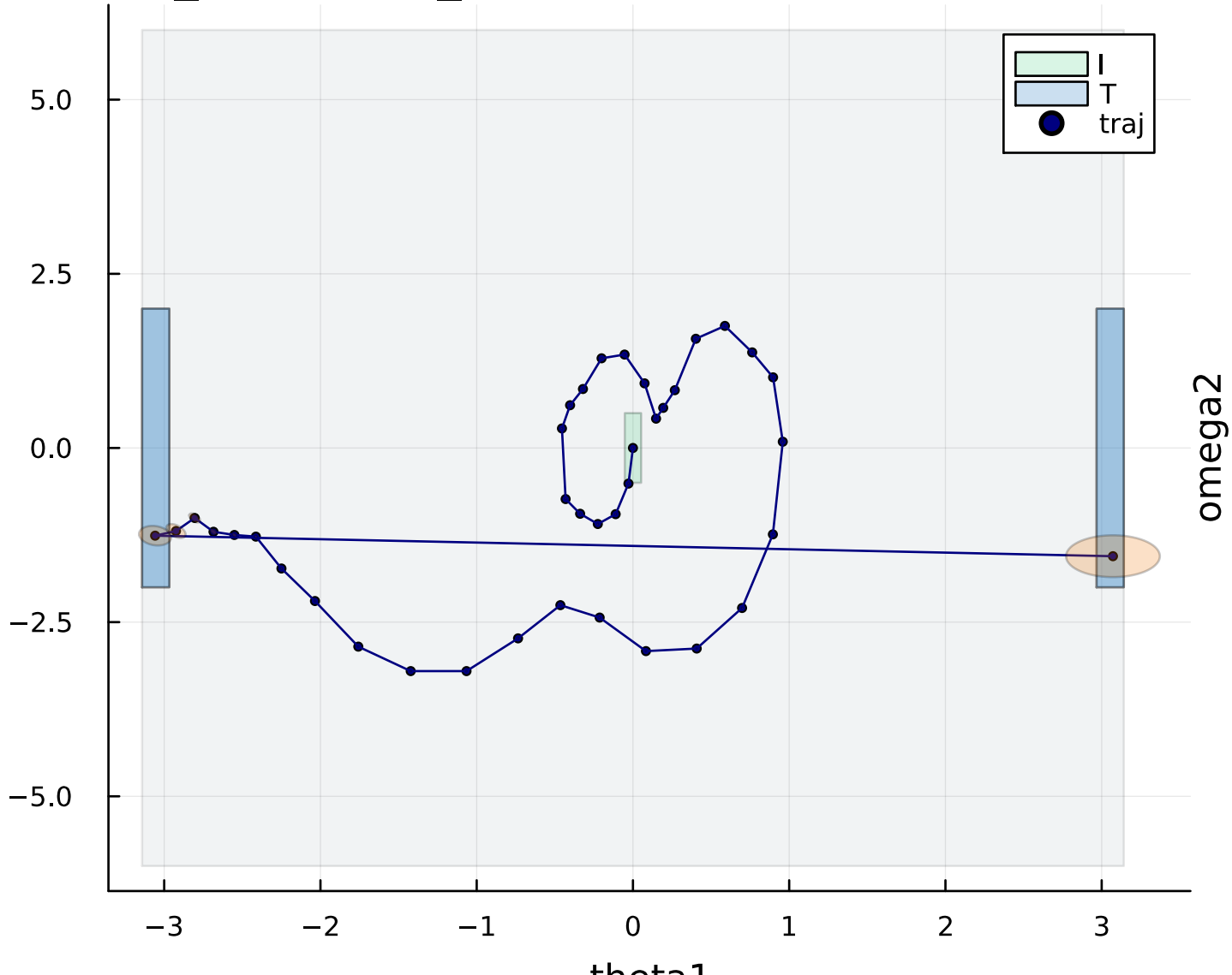
double_pendulum_mppi - certification phase portraits
