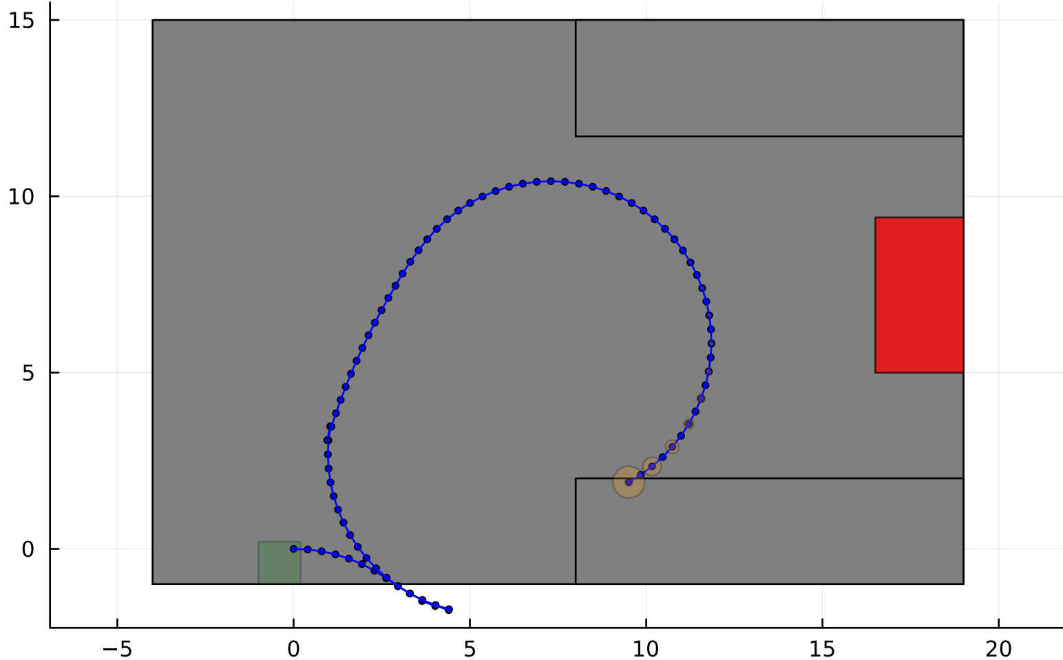
double_remorque_marche_avant_mppi (x,y)
