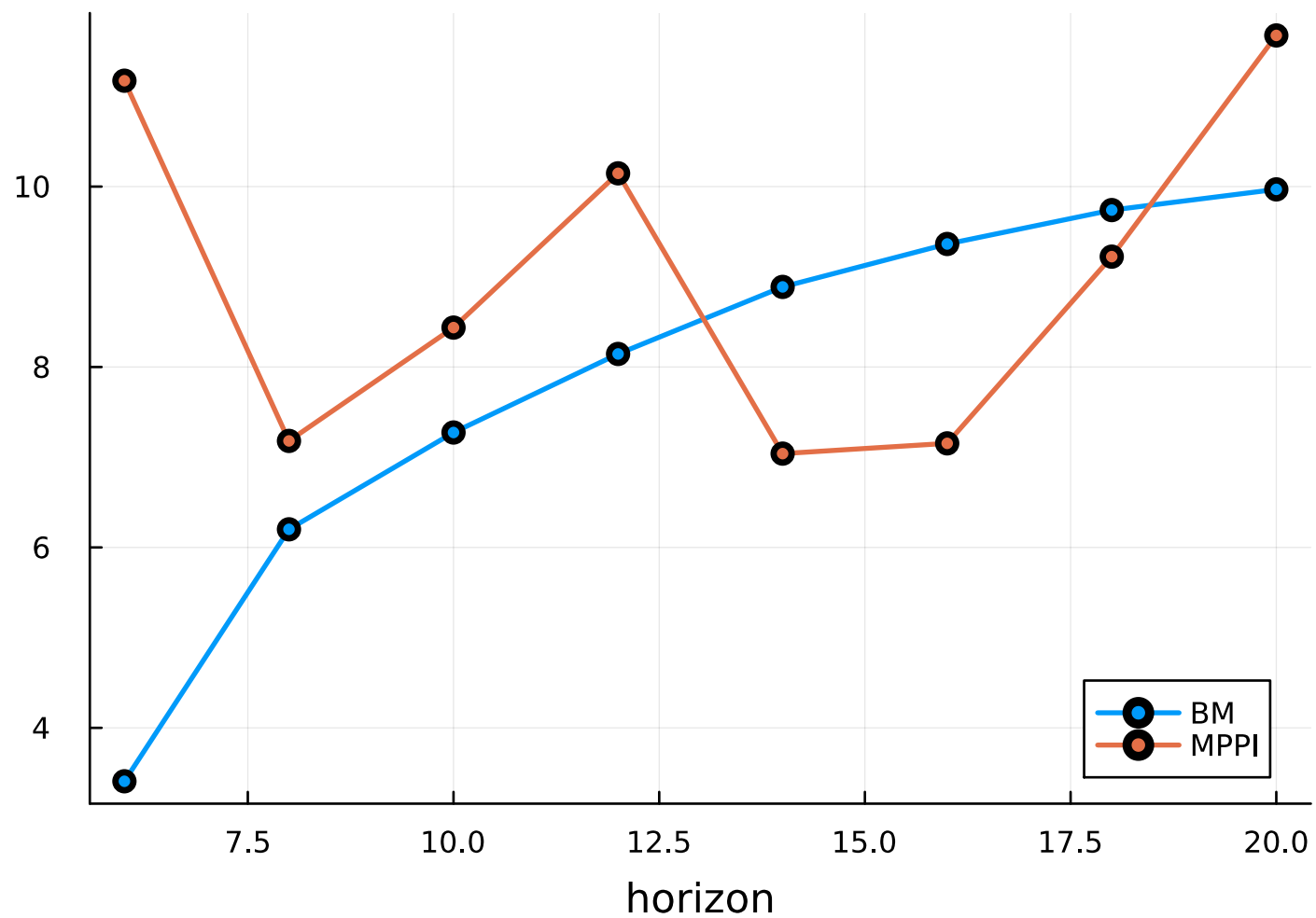
Sum ellipsoid area
