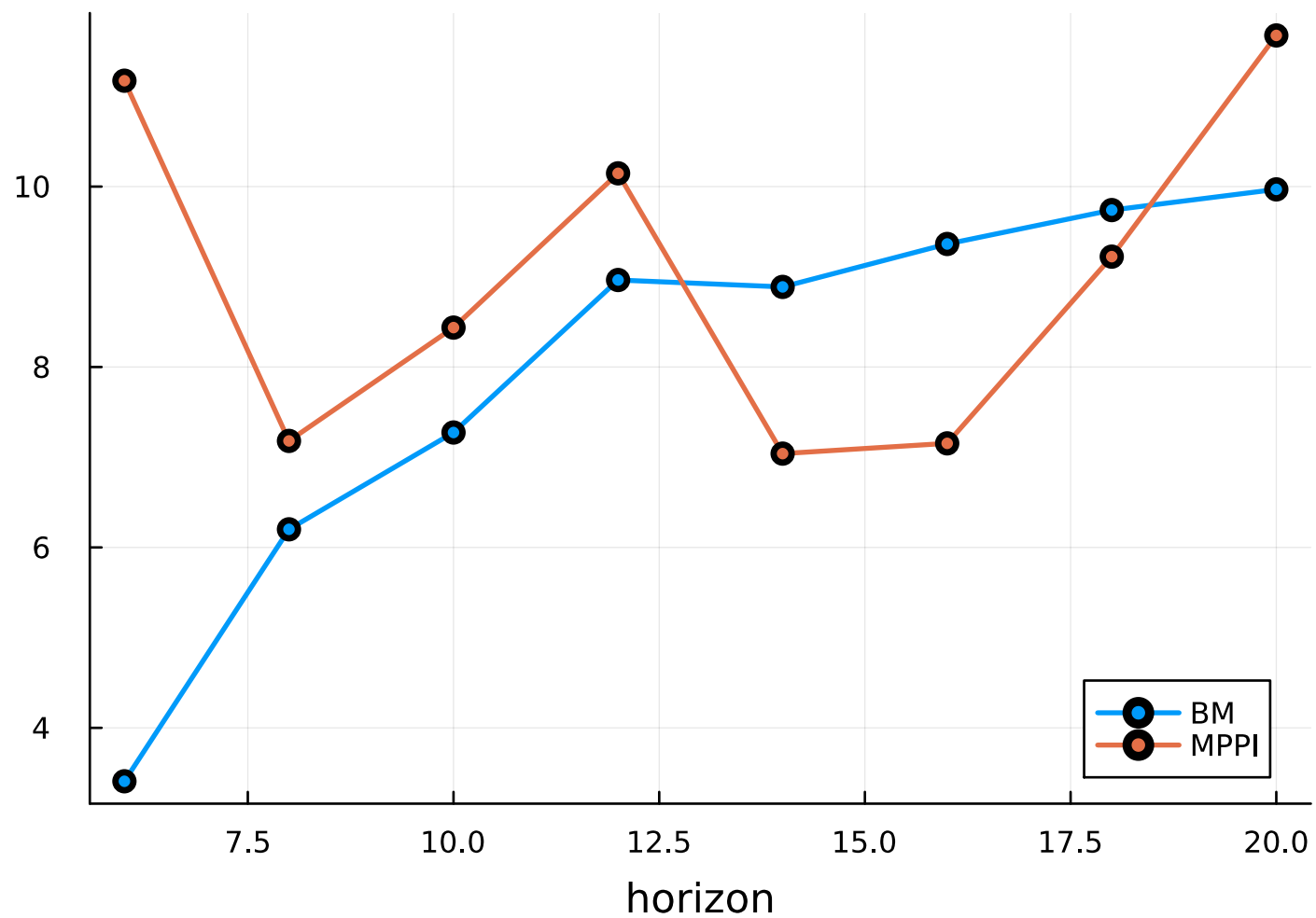
Common-prefix sum area
