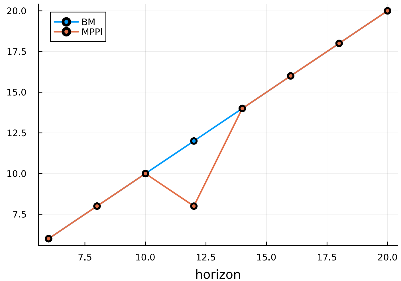
Certified steps
