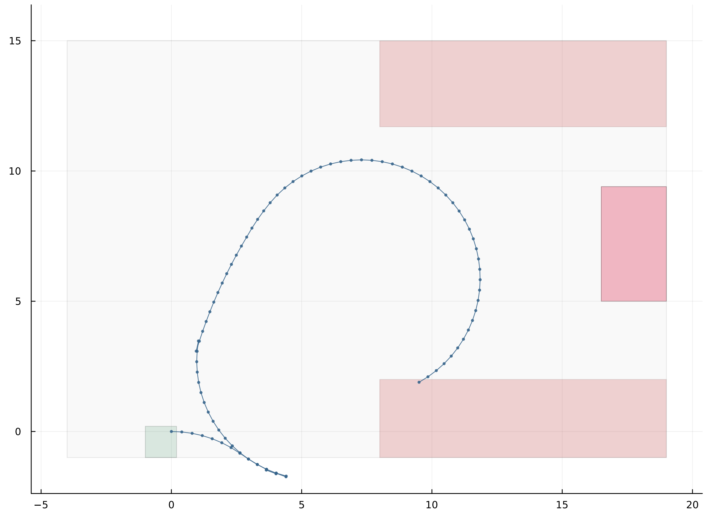
MPPI candidate traj
