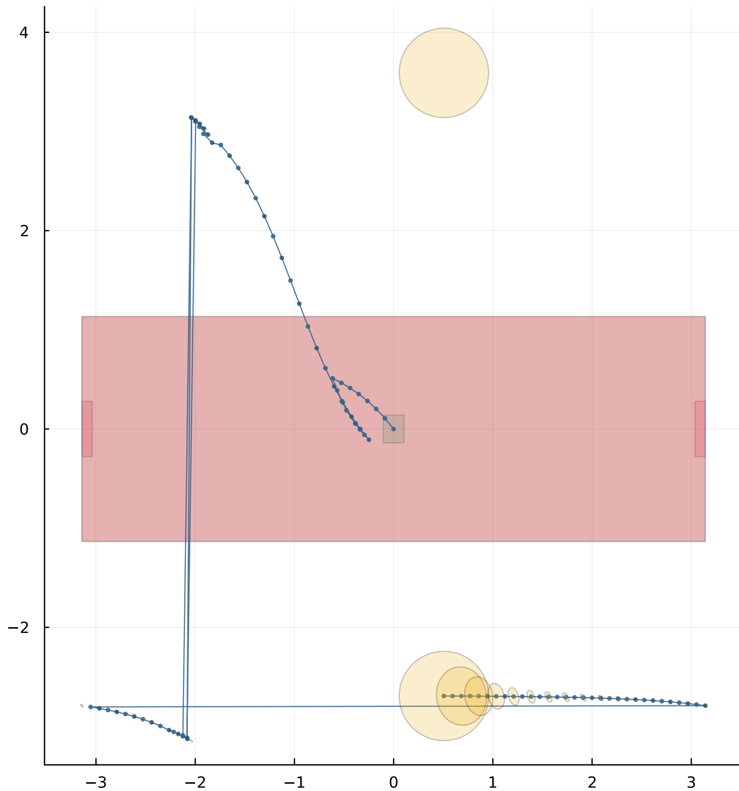
double_remorque_marche_avant_mppi (theta,phi)
