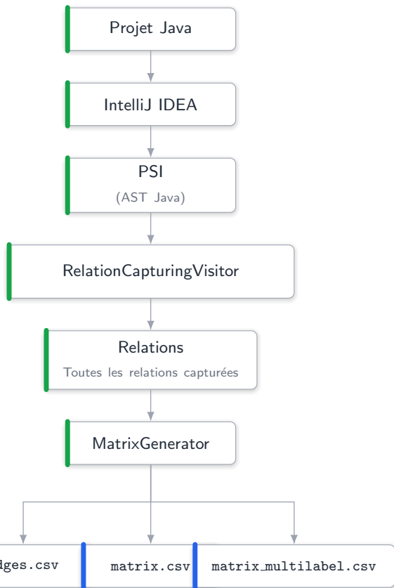
(a) Architecture du plugin
