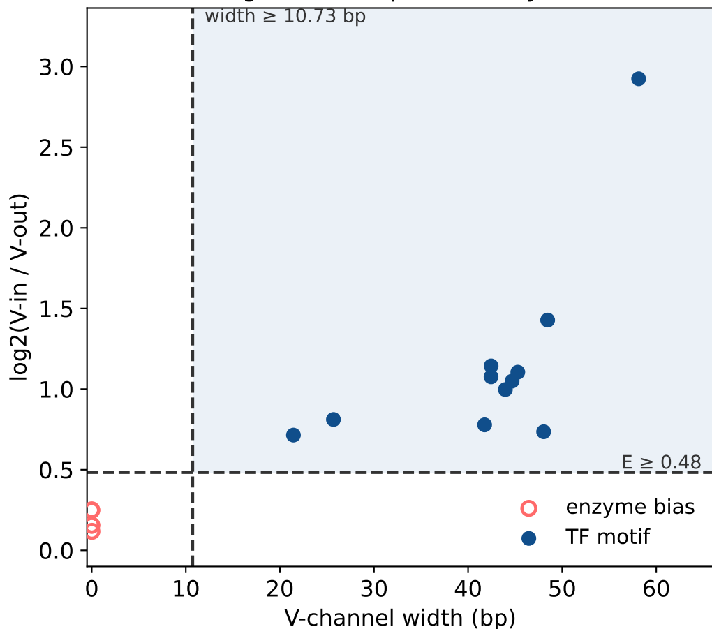
ATAC: genuine footprint vs enzyme bias
