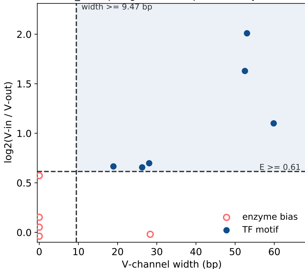
ATAC_example: genuine footprint vs enzyme bias
