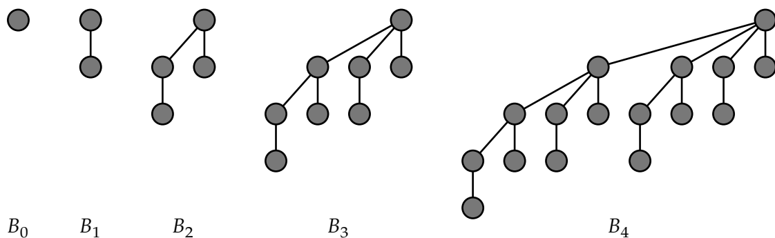
Figure 1: Binomial trees of orders 0 through 4
