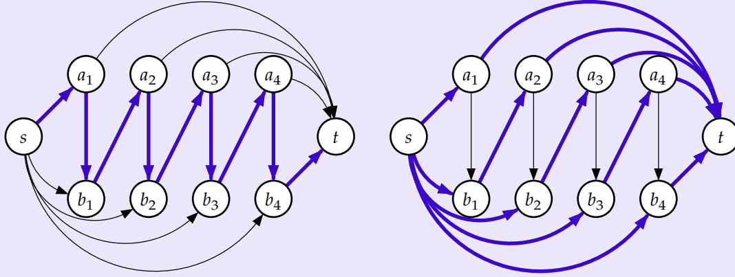
Figure 8: Construction of G_k for k = 4 . All edge capacities are 1. (a) The highlighted edges form a blocking flow f , |f| = 1 . (b) The highlighted edges form a max flow f^* , |f^*| = 5 .
