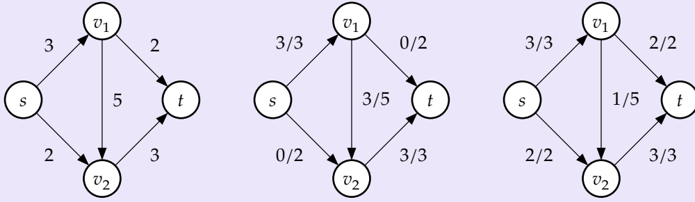
Figure 7: (a) A network G . (b) A possible flow f obtained from Forward-Edges-Only, with value 3. (c) A max flow f^* with value 5.
