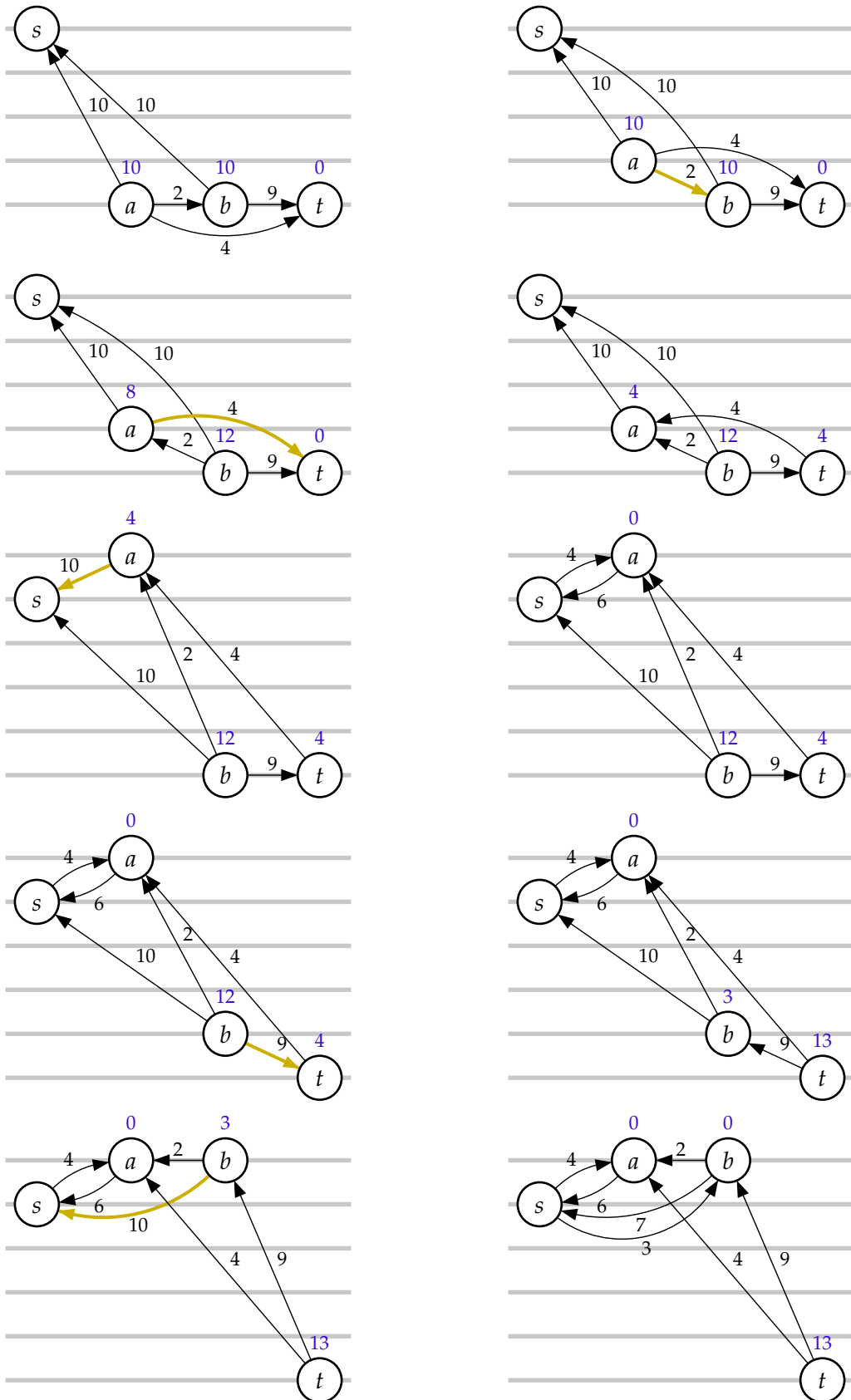
Figure 3: Working of the PUSH-RELABEL algorithm on a flow network G . Consecutive RELABEL operations on the same vertex are shown together. Excess flows are denoted by purple amounts on each vertex. Highlighted edges (in yellow) denote edges which are about to be subject to a PUSH operation.
