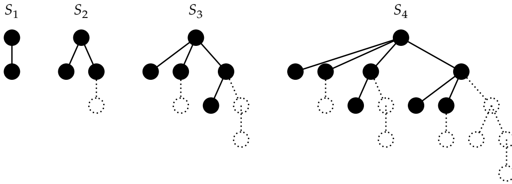
Figure 13: Minimal node trees of different degrees in a Fibonacci heap
