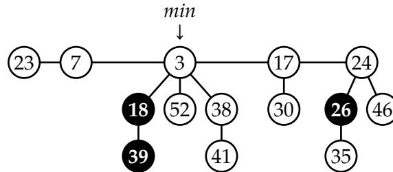
Figure 10: A fibonacci heap. Marked nodes are indicated with a dark background.
