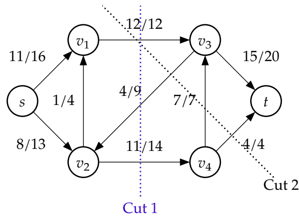
Figure 2: Two cuts (S_1, T_1) and (S_2, T_2) of G . S_1 = \{s, v_1, v_2\} . S_2 = \{s, v_1, v_2, v_4\}
