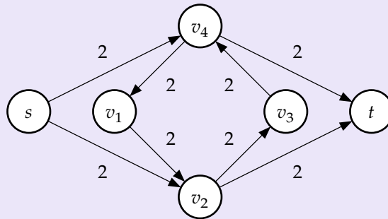
Figure 10: A network for which FORD-FULKERSON may not find a acyclic flow.
