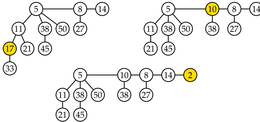
Figure: 1) DECREASE-KEY(17, 10) operation performed.
