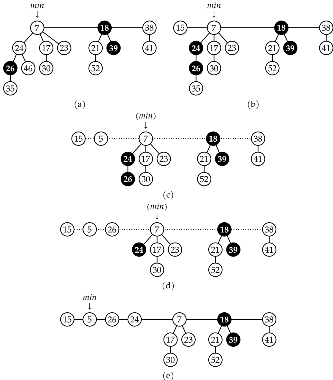
Figure: Two DECREASE-KEY operations performed on a Fibonacci Heap. b \rightarrow c \rightarrow d \rightarrow e shows how the cuts are cascaded when we have a chain of marked nodes.
