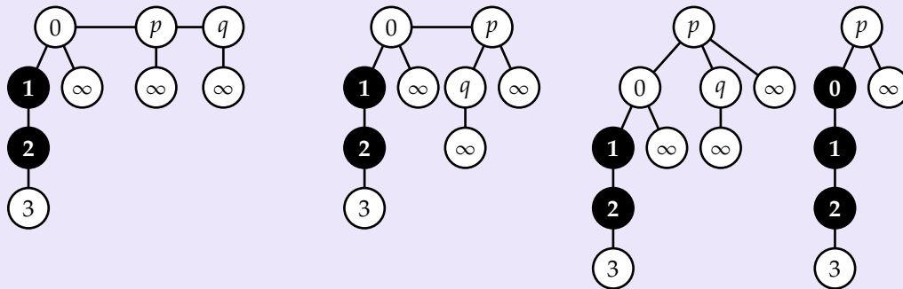
Figure: Inductive construction of a chain of marked nodes
