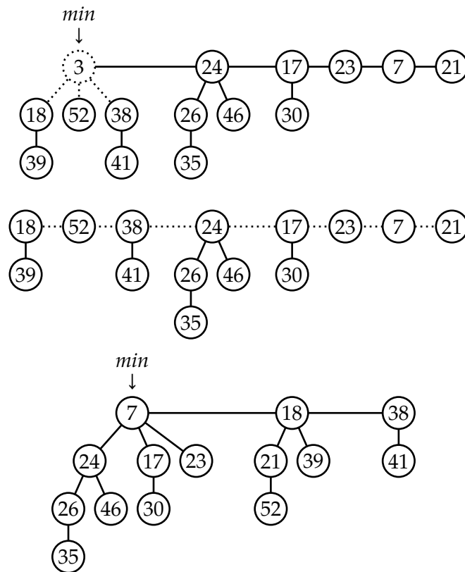
Figure: EXTRACT-MIN operation performed on a heap. Top: Initial state. Middle: State just after removing the minimum node. Bottom: Final heap after CONSOLIDATE. (For detailed steps of consolidation, see Figure 19.4, CLRS)
