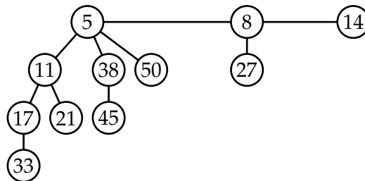
Figure: A binomial heap with n = 11 nodes, represented by a set of binomial trees B_3, B_1 and B_0
