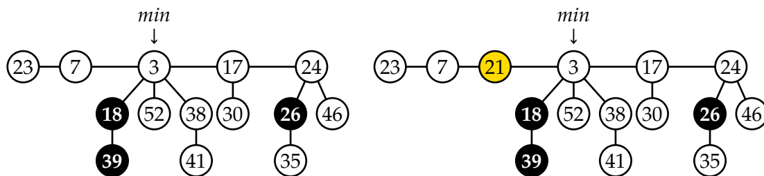
Figure: Running INSERT(21) on the Fibonacci heap.
