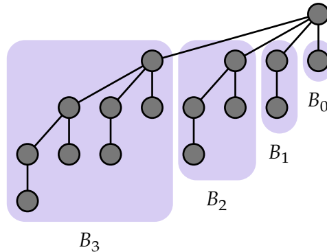
Figure: The children of B_4 are themselves binomial trees, B_0, B_1, B_2 and B_3 from right to left.
