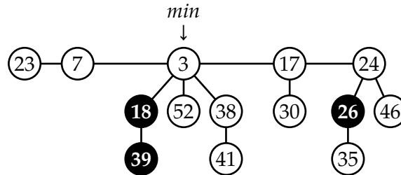
Figure: A fibonacci heap. Marked nodes are indicated with a dark background.
