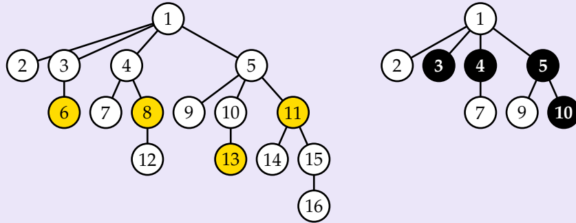
Figure: Transformation of B_4 into S_4 with F_6 = 8 nodes by Step 2
