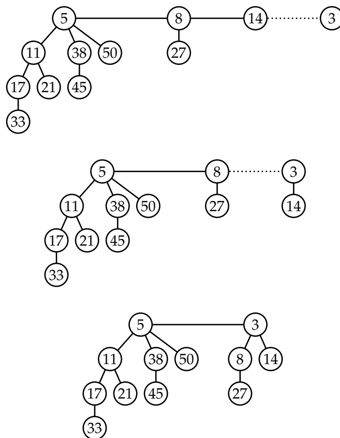
Figure: Insertion of a new node 3 to the binomial heap. The resulting heap is of size n = 12 .
