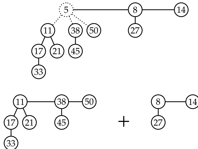
Figure: Deletion of the min key node (5) from the binomial heap
