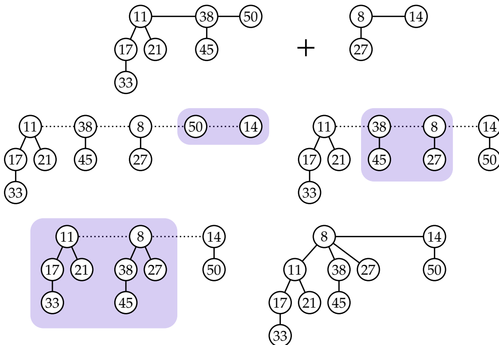
Figure: Union of two binomial heaps
