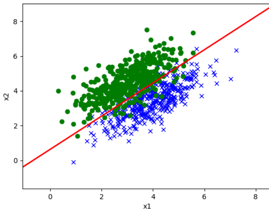
(f) Dataset 1:
