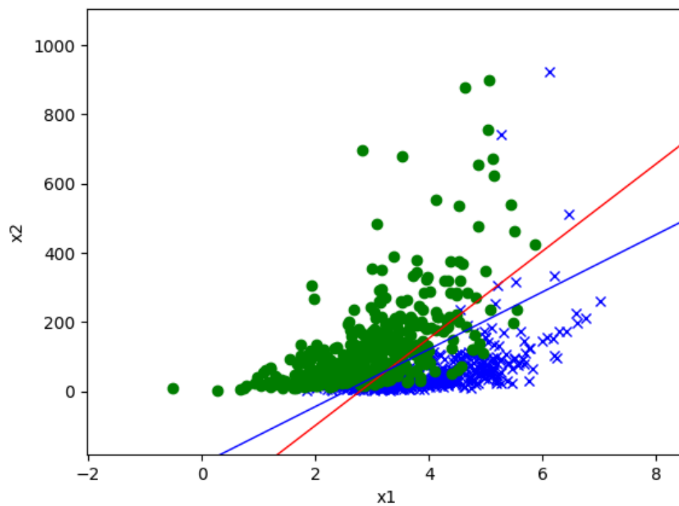
(g) Dataset 2:
