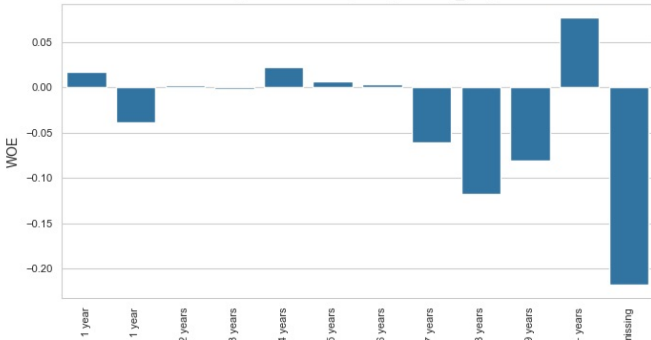
Weight of Evidence (WOE) for emp_length
