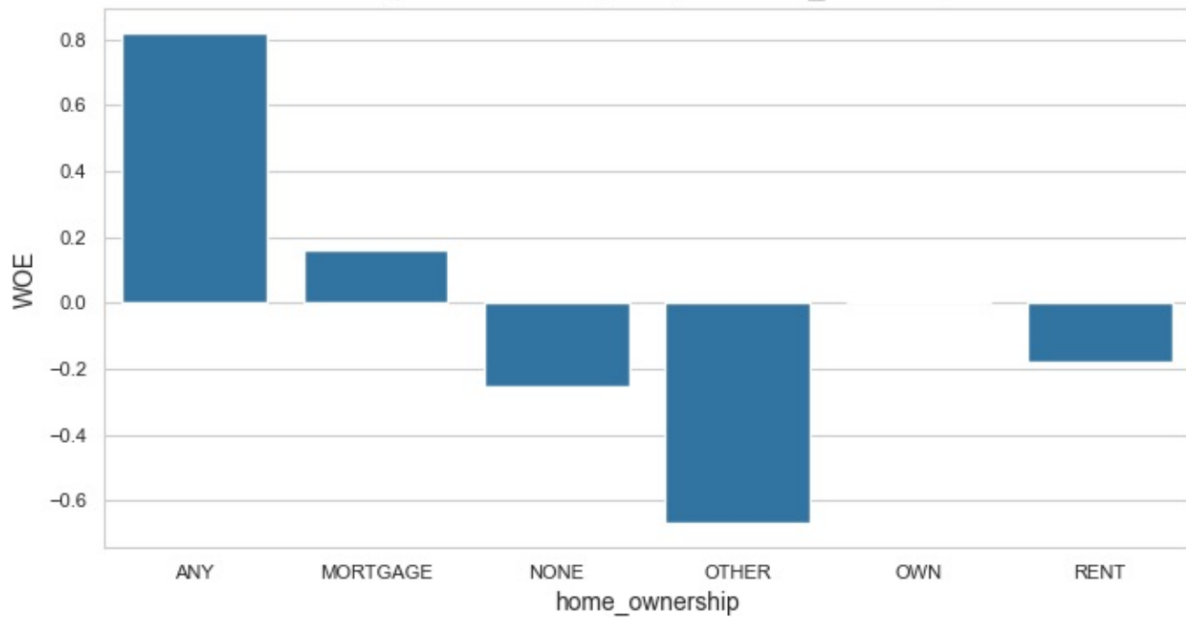
Weight of Evidence (WOE) for home_ownership
