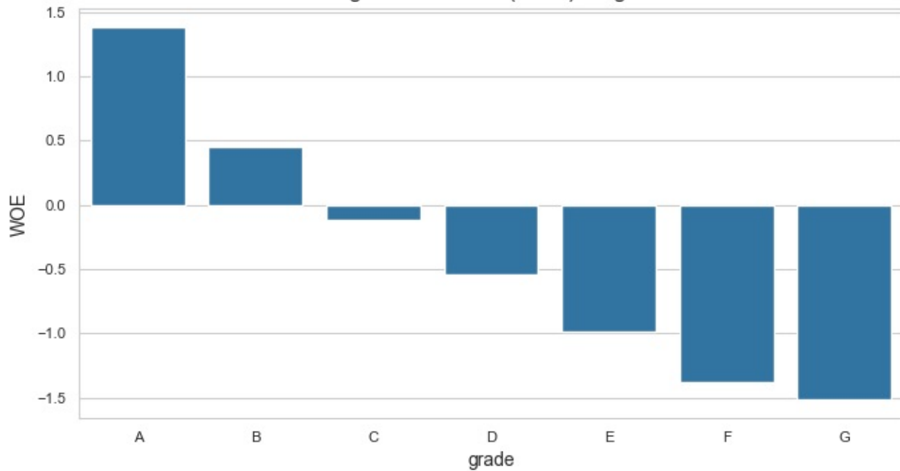
Weight of Evidence (WOE) for grade
