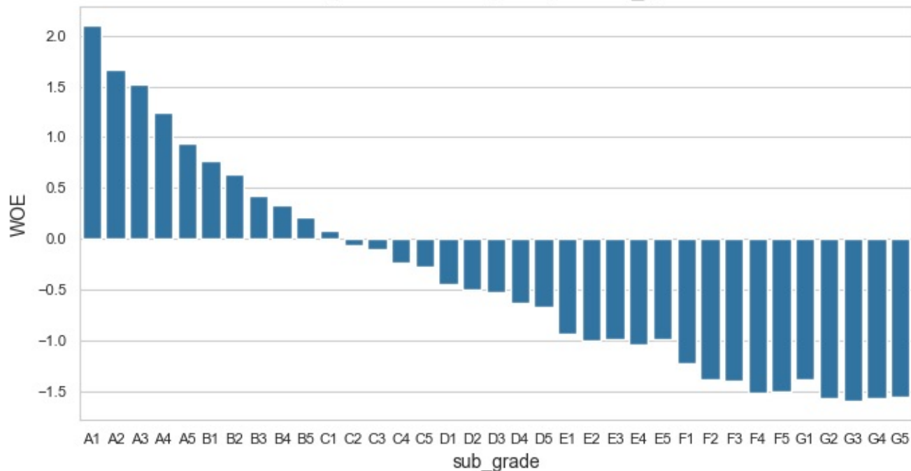
Weight of Evidence (WOE) for sub_grade
