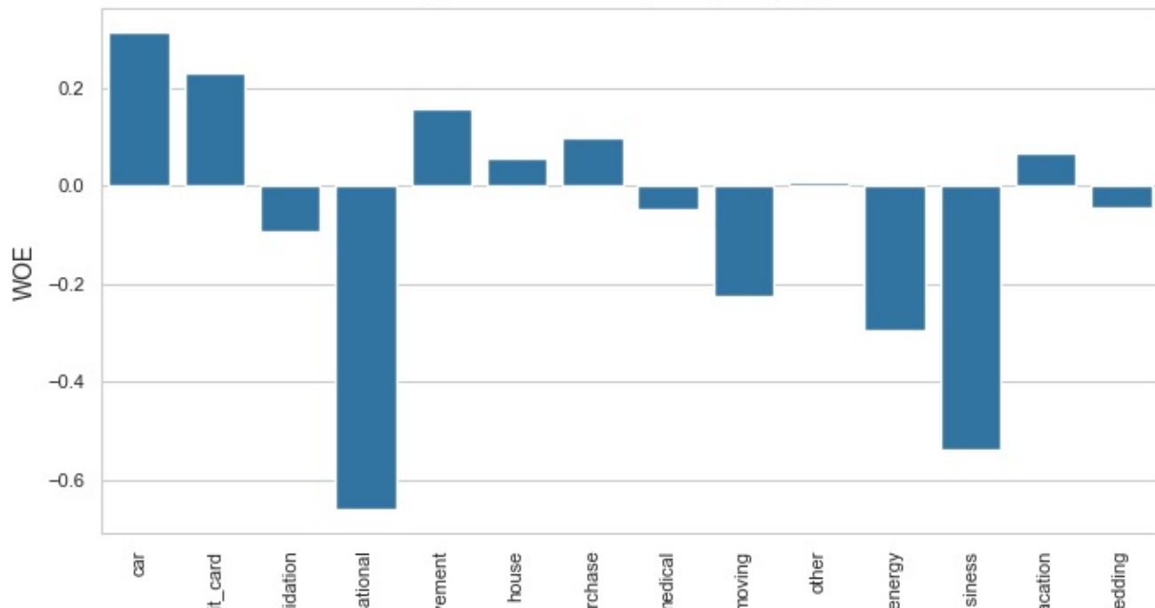
Weight of Evidence (WOE) for purpose
