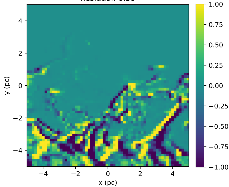
Predicted Source Term (FNN) Residual: 0.59
