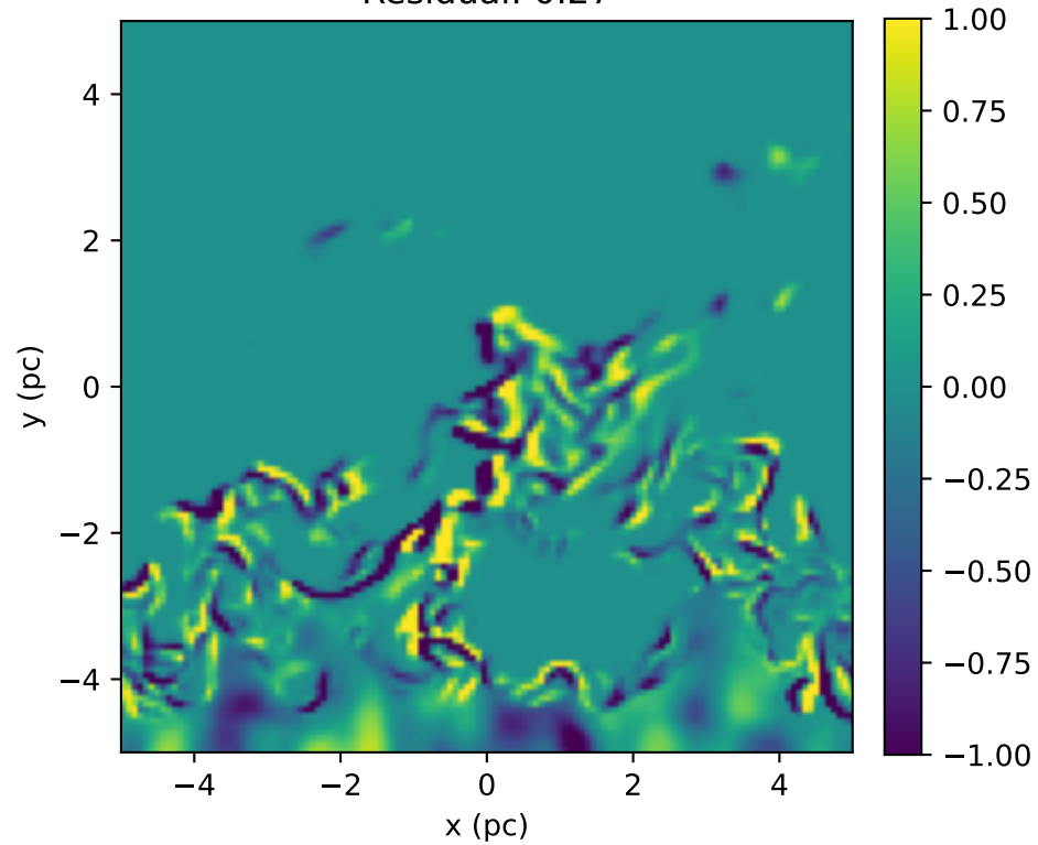
Predicted Source Term (CNN) Residual: 0.27
