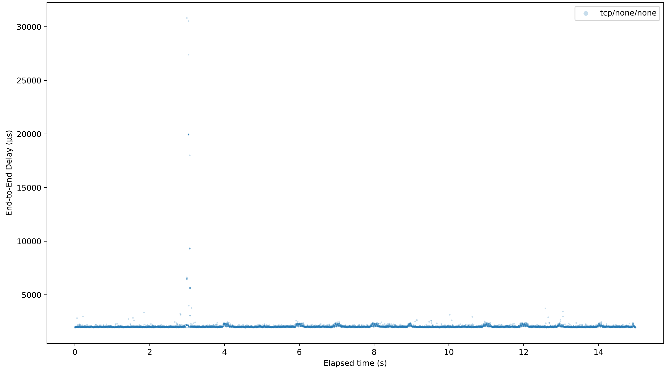
End-to-End Delay per Packet
