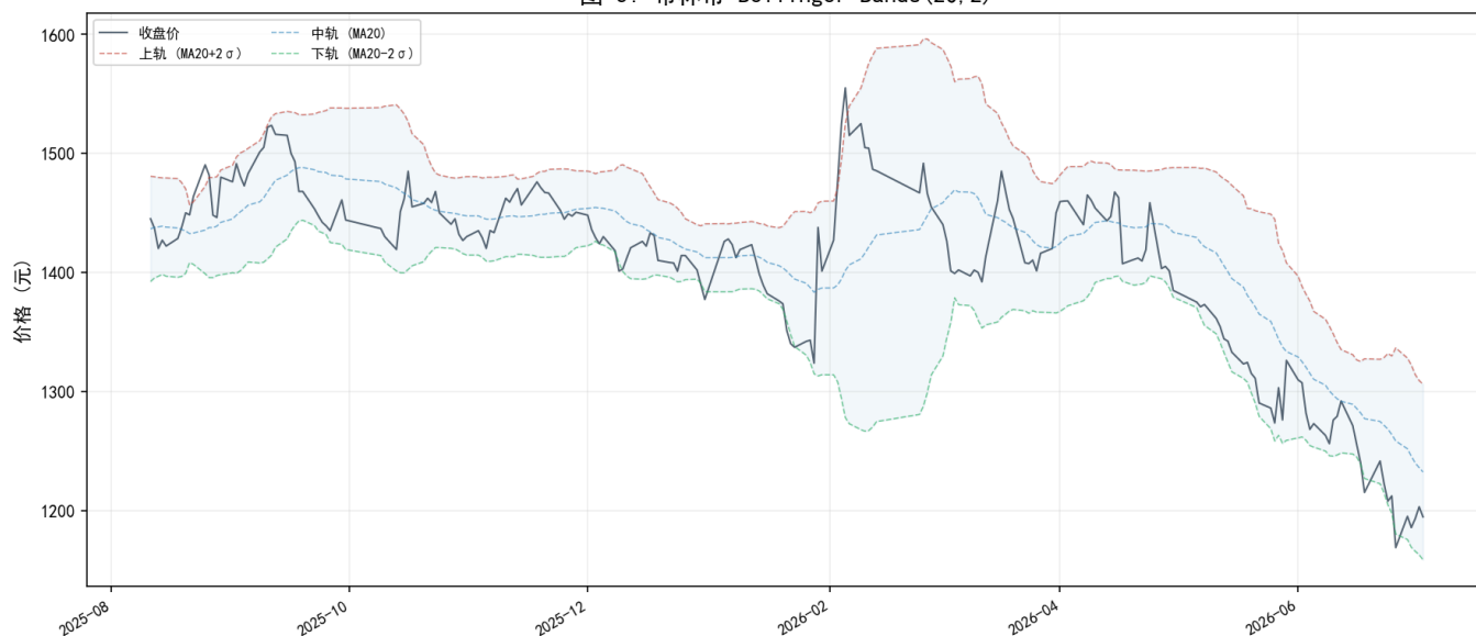
图 3：布林带 Bollinger Bands (20, 2)
