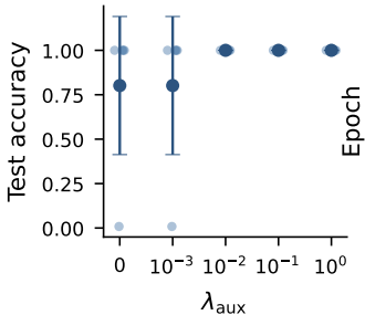
Final accuracy
