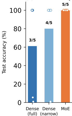
(a) Final accuracy
