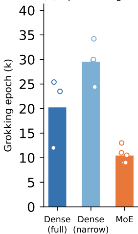
(b) Epochs to grok
