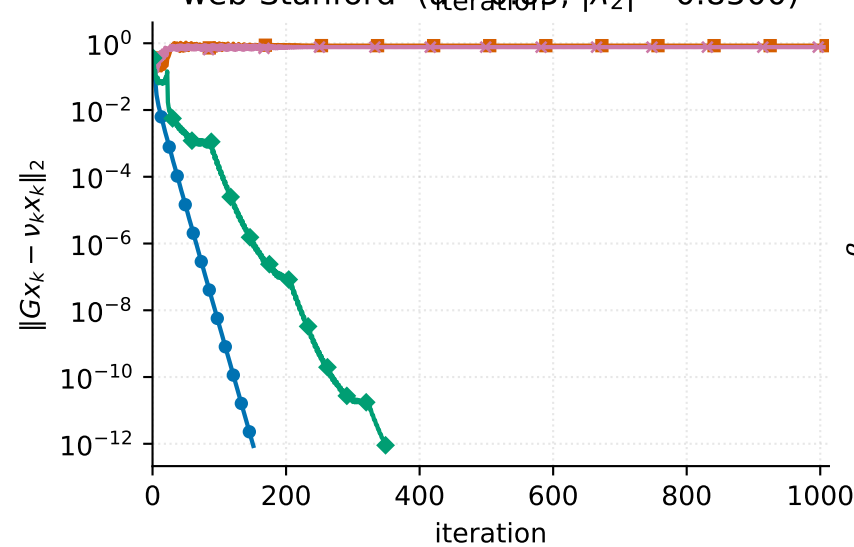
web-Stanford ( d = 0.85 , |\lambda_2| = 0.8500 )
