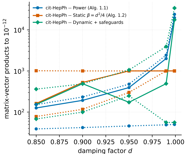
Cost of ranking as the spectral gap closes
