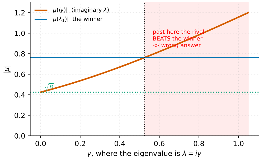
...but imaginary eigenvalues escape upward (this is what breaks PageRank)
