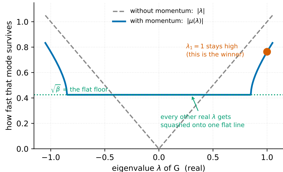
Momentum works by flattening the rivals (real eigenvalues)
