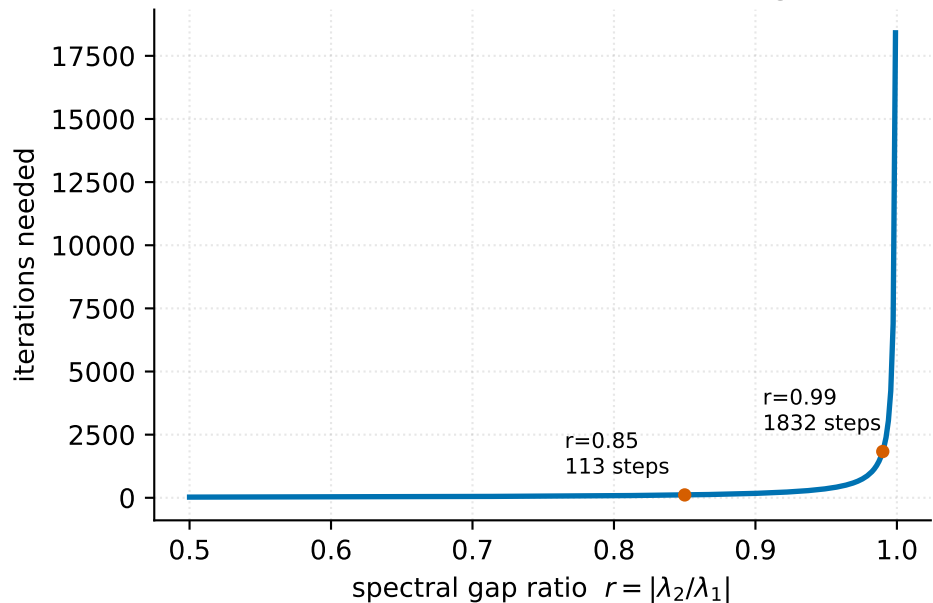
The closer r is to 1, the slower it gets
