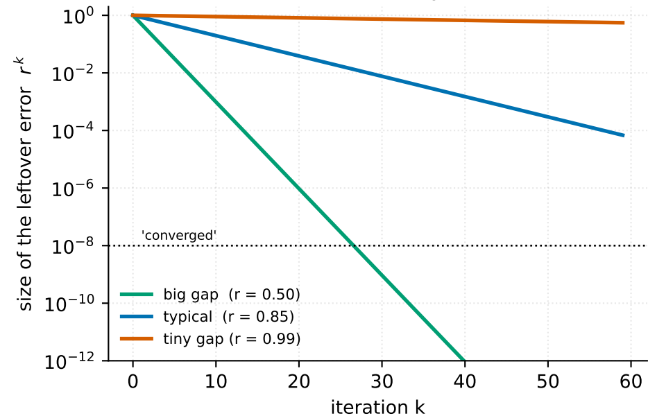
Power iteration: error shrinks by a factor r each step
