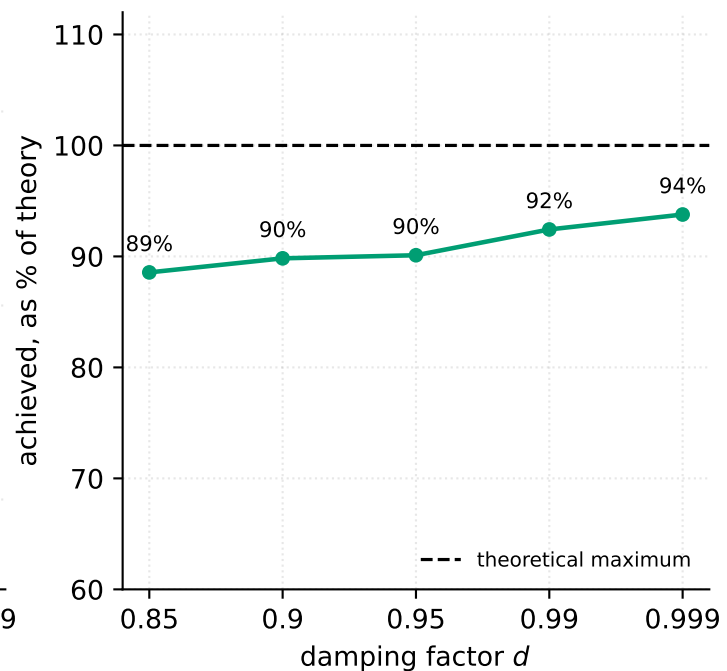
Alg. 3.1 attains 89-94% of the theoretical maximum
