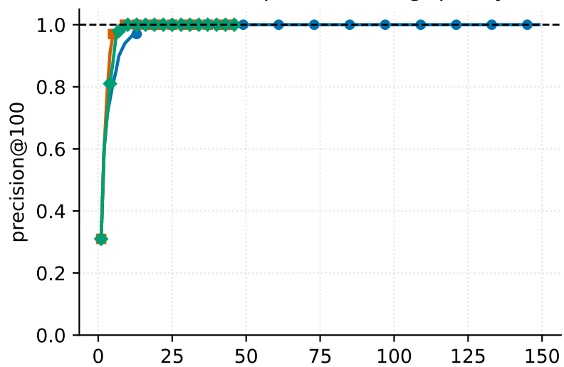
d = 0.99 : top-100 ranking quality
