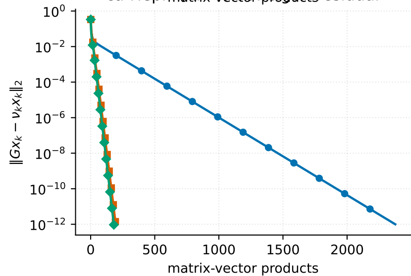
ca-HepPh, d = 0.99 : eigen-residual
