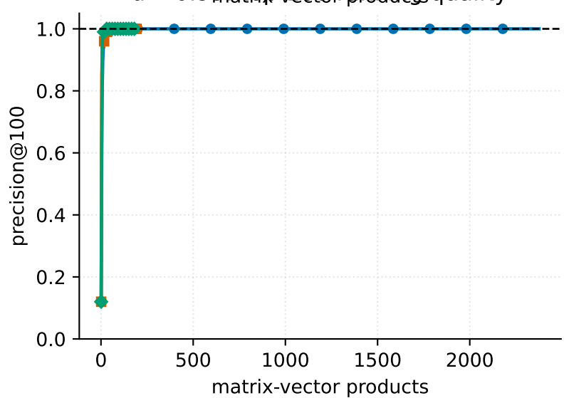
d = 0.99 : top-100 ranking quality
