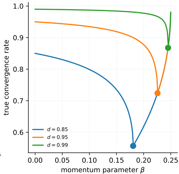
C. \beta = d^2/4 (dots) sits at the minimum of the true rate curve
