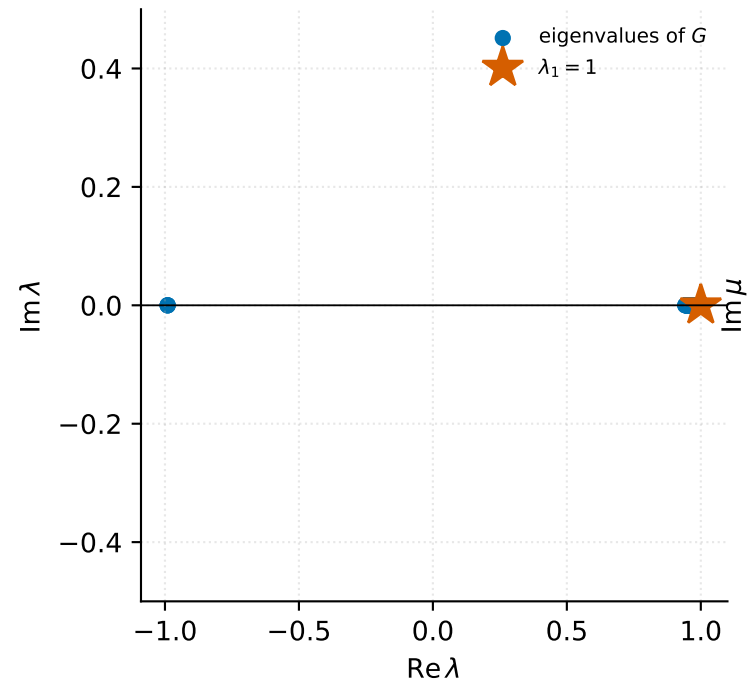
A. The spectrum is real d = 0.99 , \max |\operatorname{Im} \lambda| = 5.2\text{e-}16
