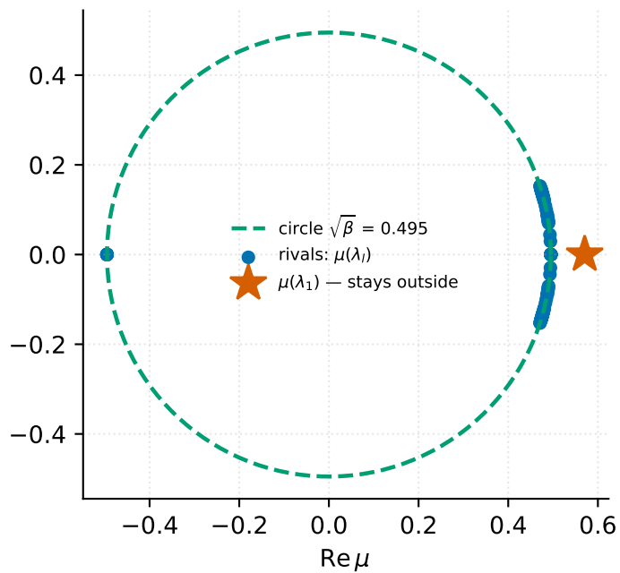
B. Momentum folds every rival onto one small circle
