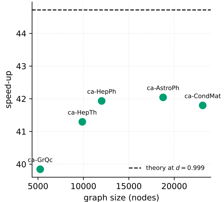
Independent of graph size ( d = 0.999 )
