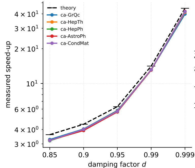
All five undirected graphs follow the same curve
