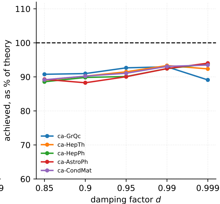
Alg. 3.1 attains a consistent fraction of the maximum
