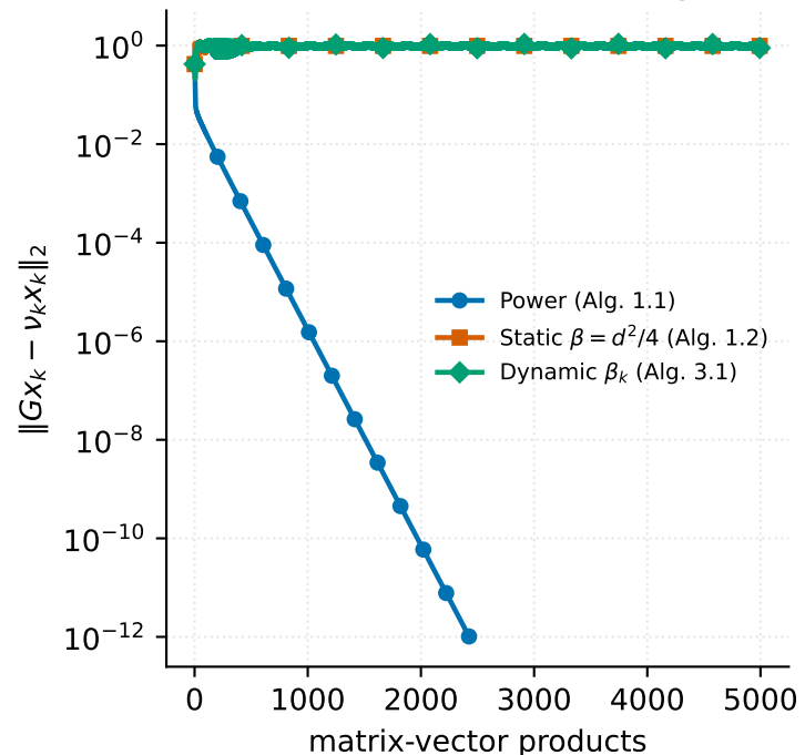
C. web-Stanford, d = 0.99 : momentum never converges
