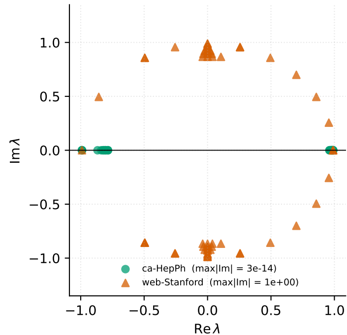
A. Undirected stays on the real axis; directed does not ( d = 0.99 )
