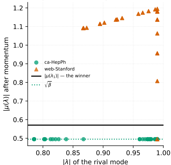
B. Real rivals land on \sqrt{\beta} ; complex ones climb past the winner
