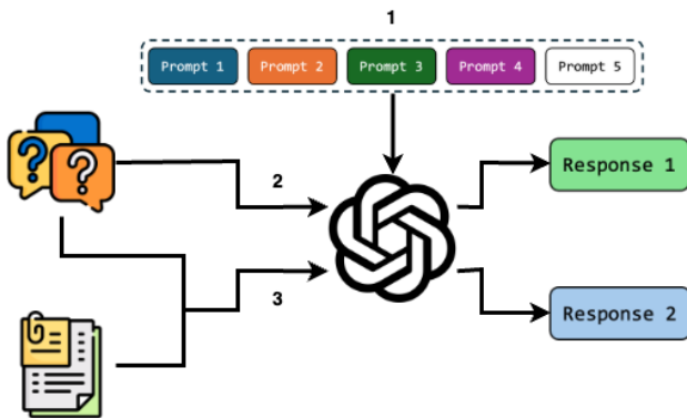
Figure 2: Prompt, LLM, and RAG pipeline.
