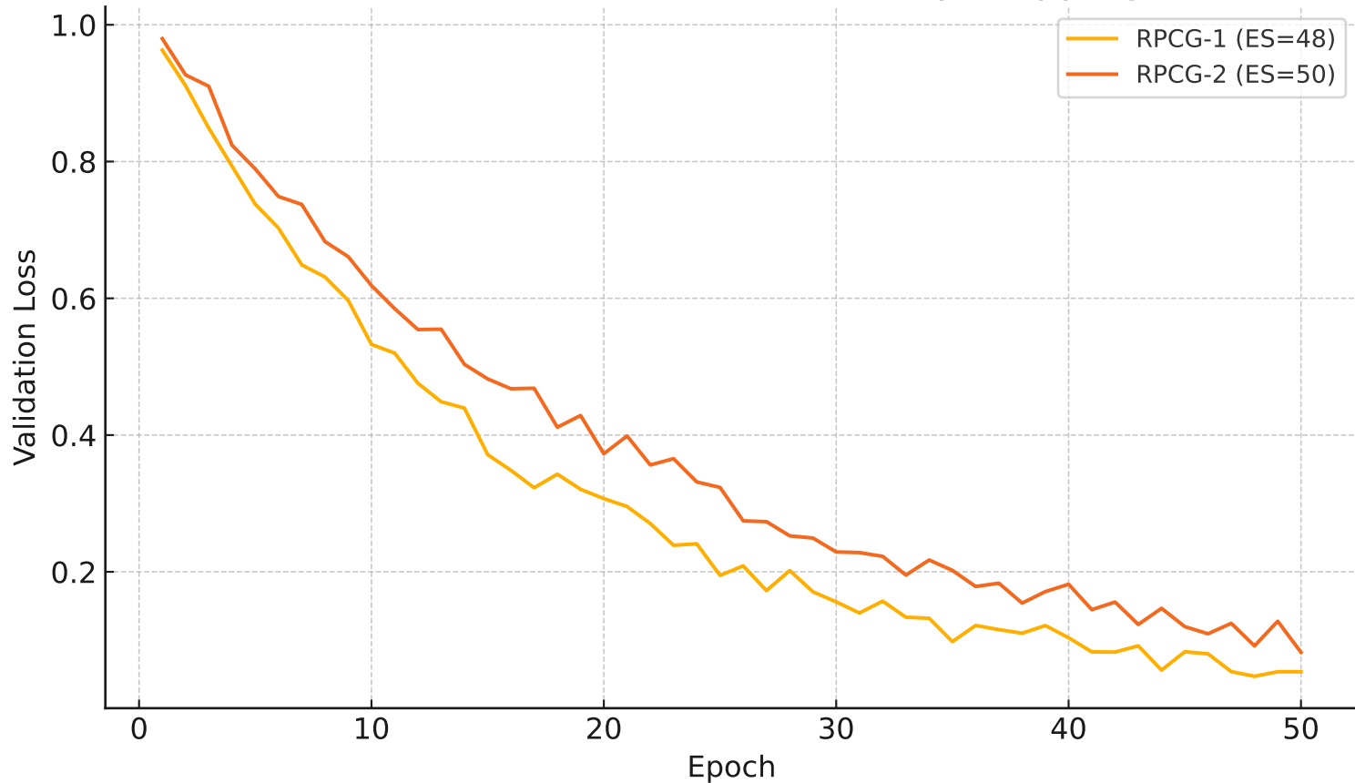
Validation Loss Curves with Early Stopping
