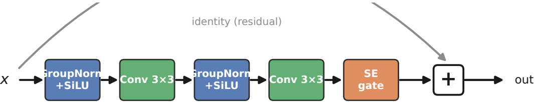
(b) Residual squeeze-excite block (repeated unit)
