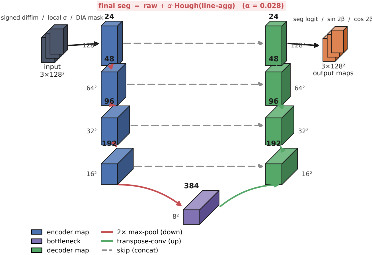
(a) Segmentation network — U-Net-ResSE with orientation + learnable Hough aggregator
