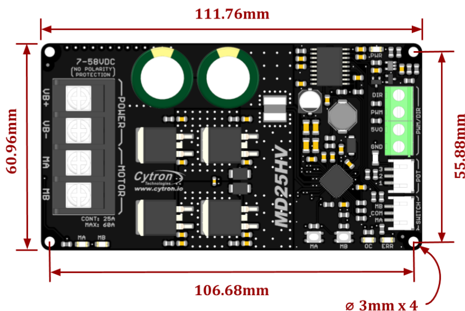
Figure 2: MD25HV Dimension
