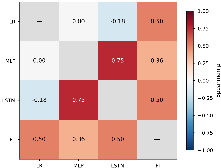
Cross-model rank agreement (Spearman \rho ) on occlusion importances
