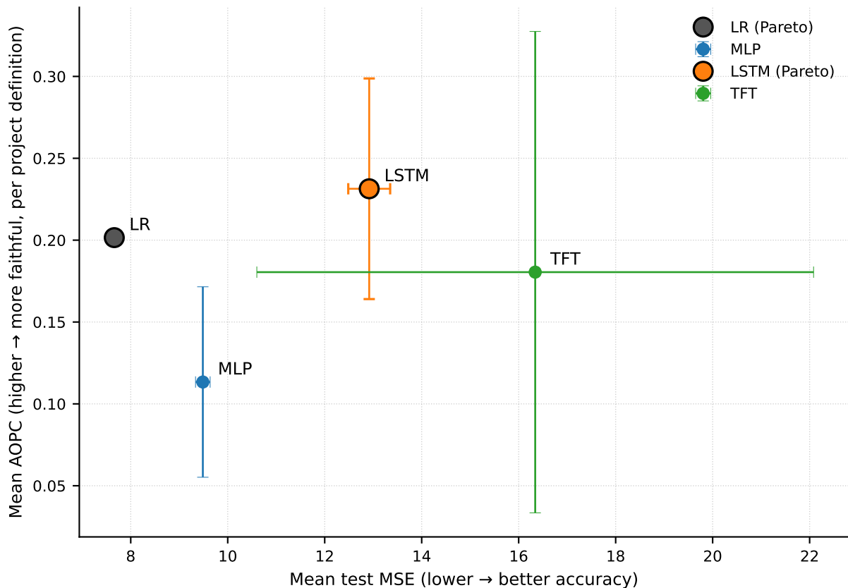
Accuracy vs. occlusion-based faithfulness — present configuration
