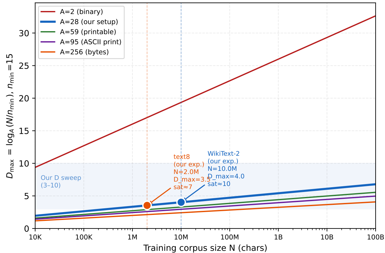
Theoretical Saturation Depth vs. Corpus Size
