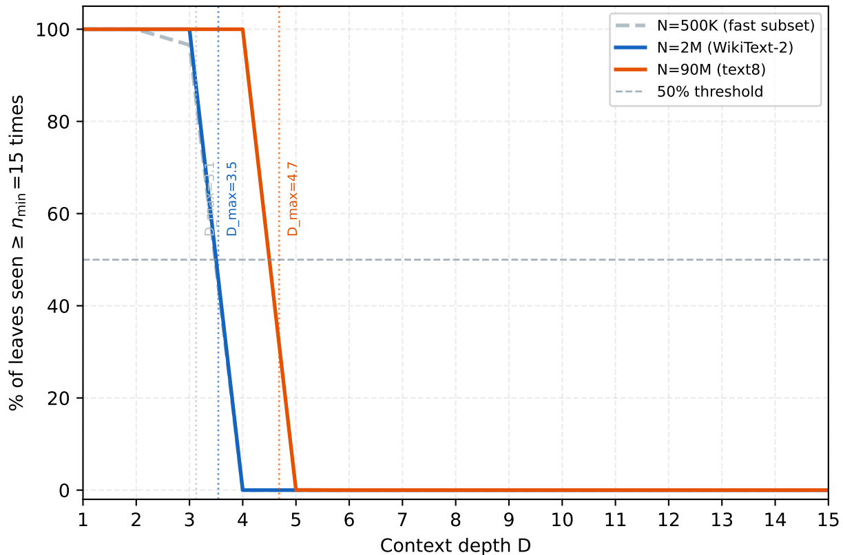
Coverage: Fraction of Useful Leaves vs. Depth
