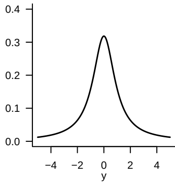
C(y;0,1)
