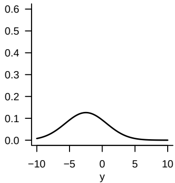
N(y;-2.5,10)
