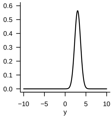
N(y;3,0.5)
