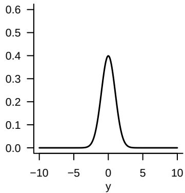
N(y;0,1)
