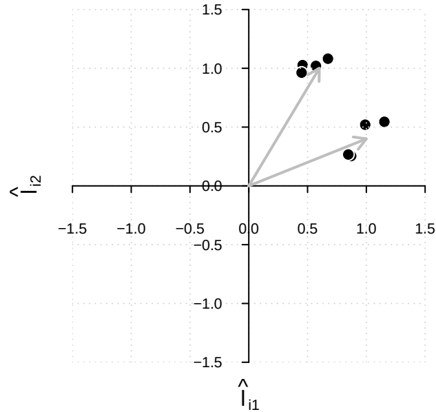
"Oblique Rotation"
