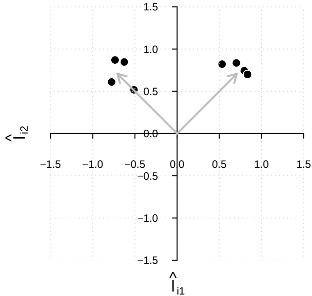
"Orthogonale Rotation"
