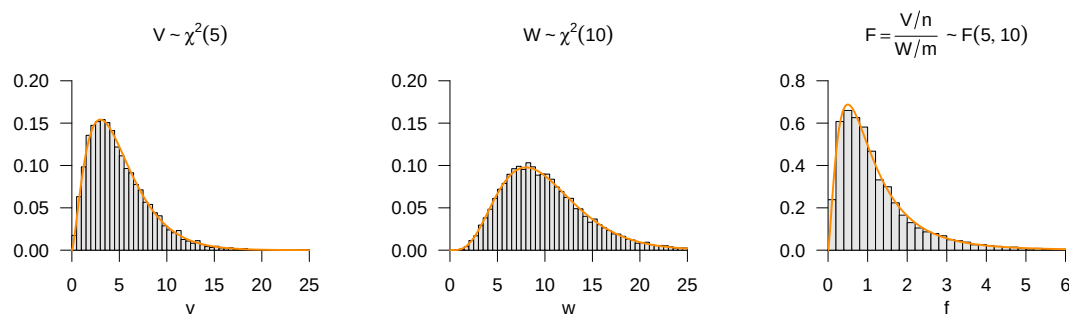
Figure 29.19 F -transformation of normally distributed random variables.
