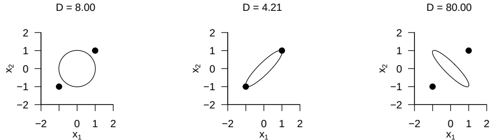
Figure 45.2 Mahalanobis distances as a function of component covariances.
